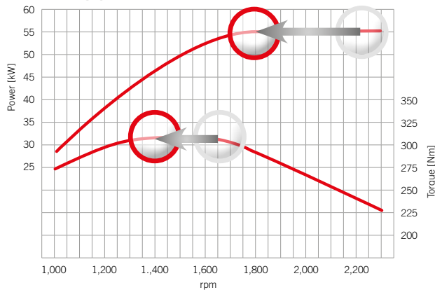
FARMALL 75 C
